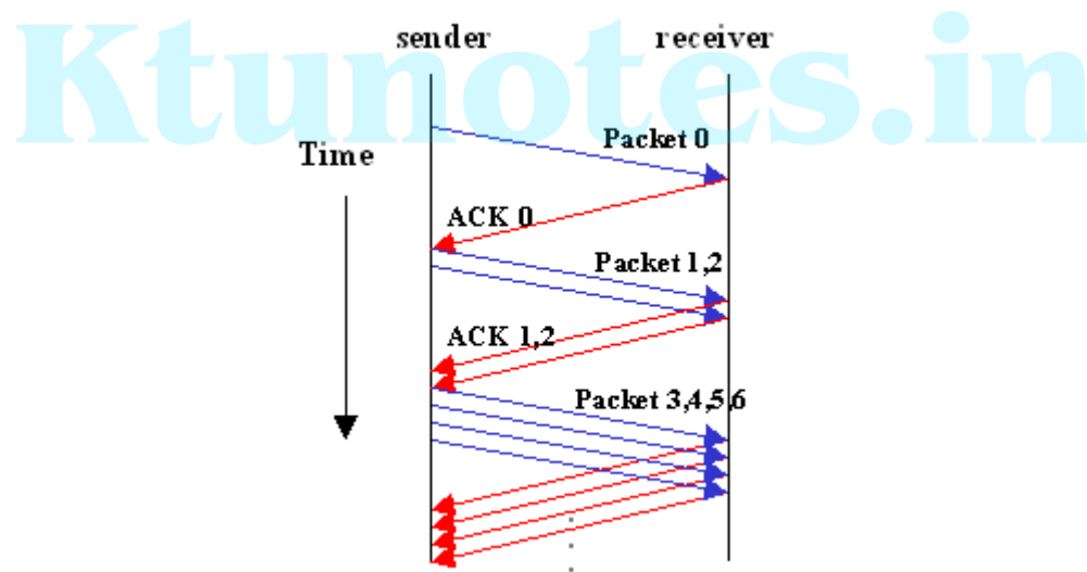
Fig.4.6 Slow start
