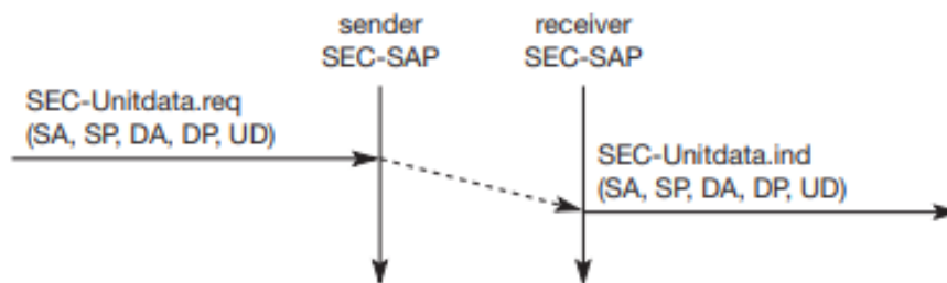
Fig.4.13 WTLS datagram transfer
