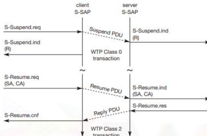
Fig.4.19 WSP/B session suspension and resume
